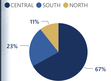
By Location, 2025
