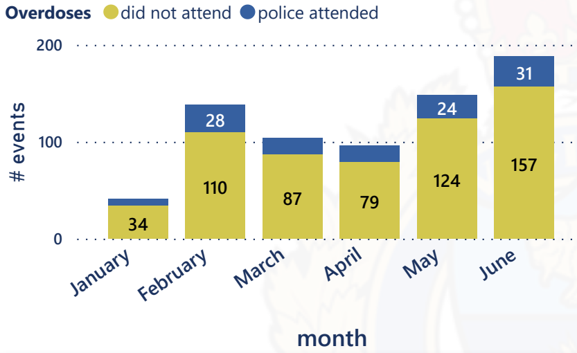
Overdose Events, 2025
