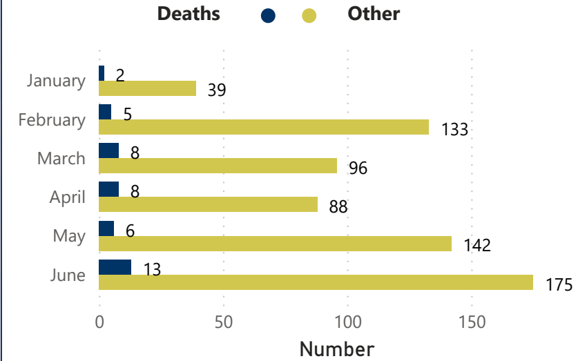
Overdose Events, 2025
