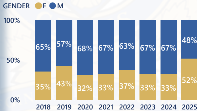
Apparent Deaths, 2018-2025
